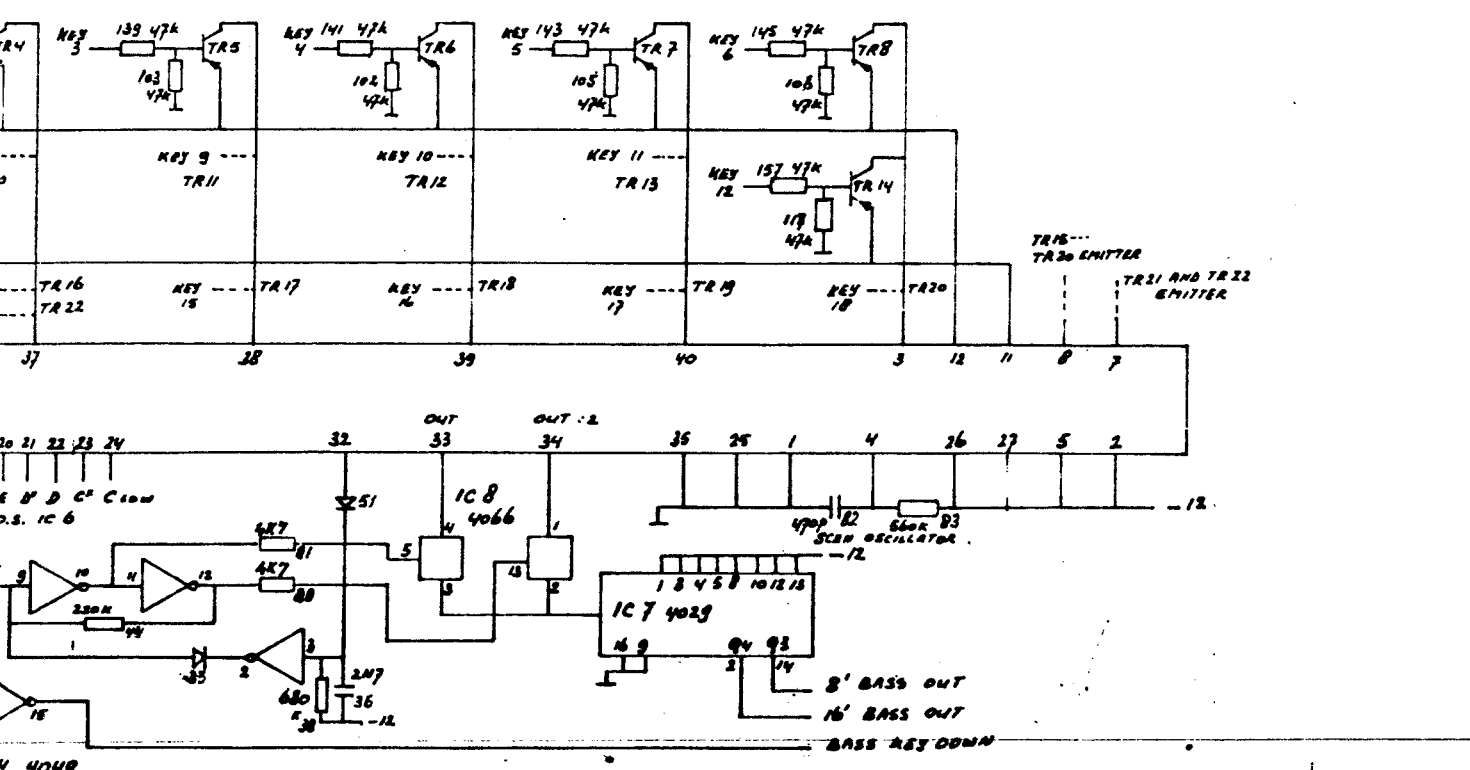
BASS LOWEST KEY DETECTION
